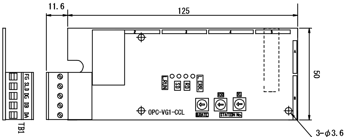
Figure 1.2-1 External Appearance
