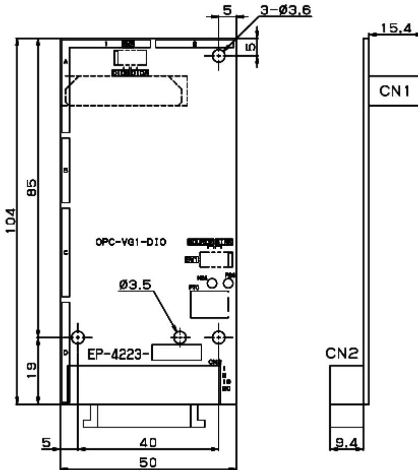
Figure 1.2-1 External Appearance
